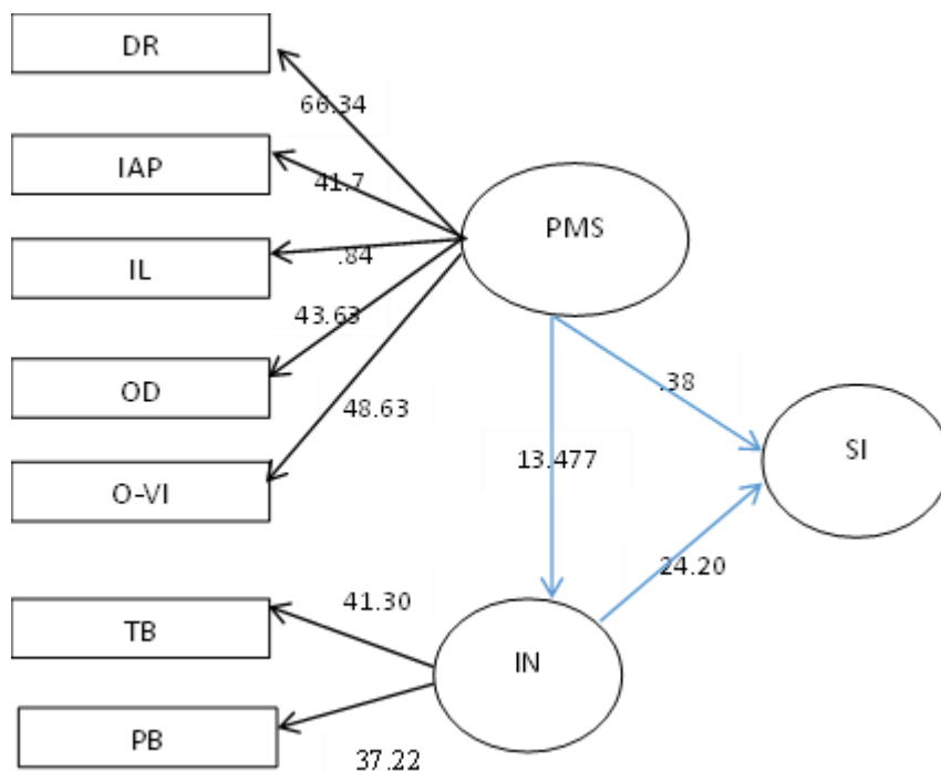
Figure 2. Significant numbers of the structural model of the research
