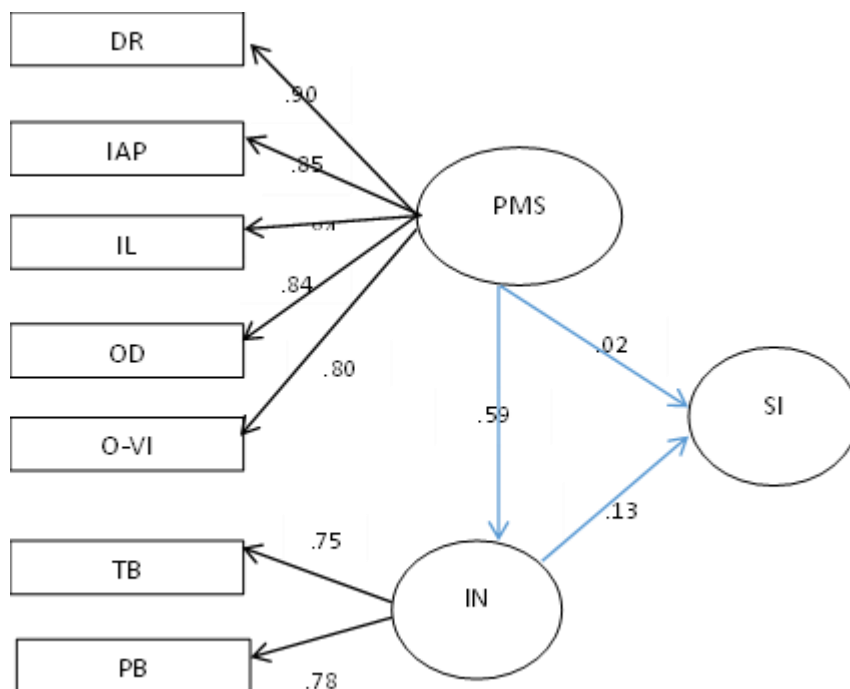
Figure 1. Standard estimation coefficients of the research structural model
