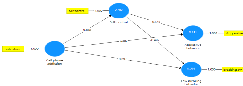
Figure 4: The amount of R^2 variables
